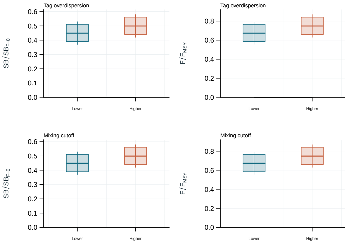
Figure 65: Weighted distributions of management quantities by design setting. Boxes: interquartile range; line: median; whiskers: 2.5th and 97.5th weighted percentiles.
