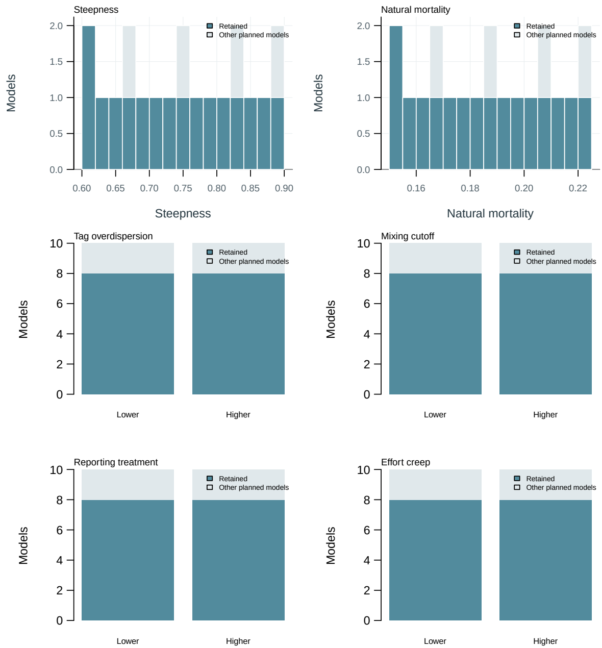
Figure 63: Planned and retained model inputs.
