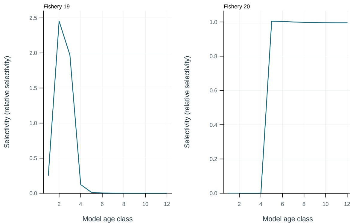
Figure 45: Fishery selectivity at age.
