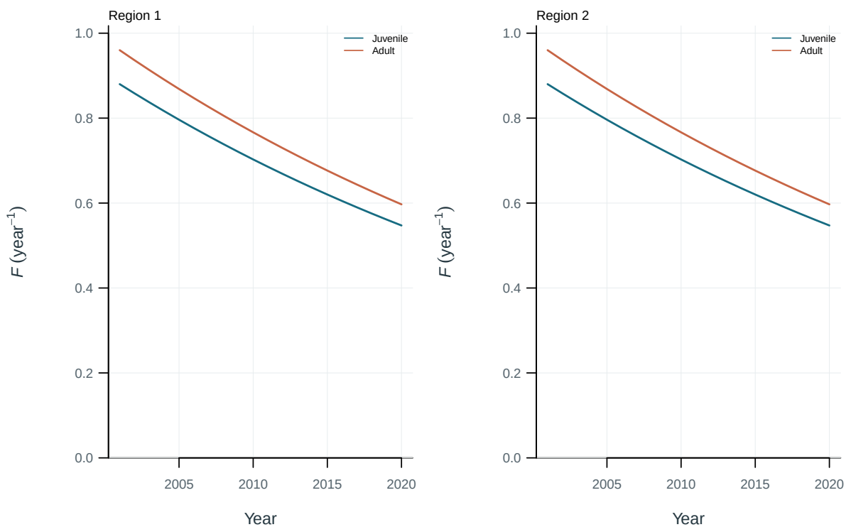
Figure 54: Illustrative output. Fishing mortality by life stage and region.
