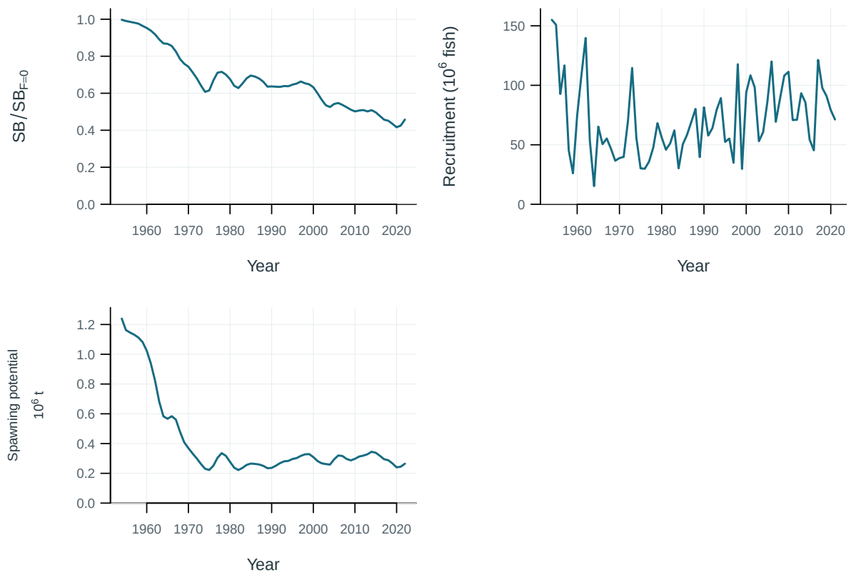
Figure 41: Estimated population trajectories.
