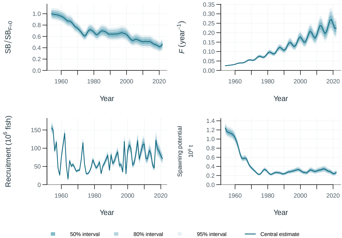
Figure 68: Population trajectories with supplied uncertainty intervals. Central 50, 80, 95% intervals (illustrative model spread and parameter perturbations).
