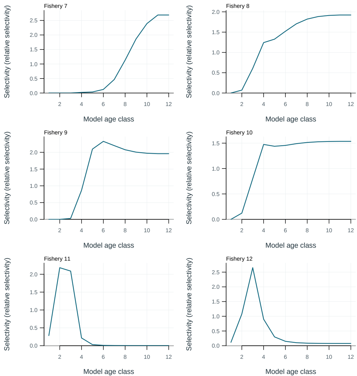
Figure 43: Fishery selectivity at age.
