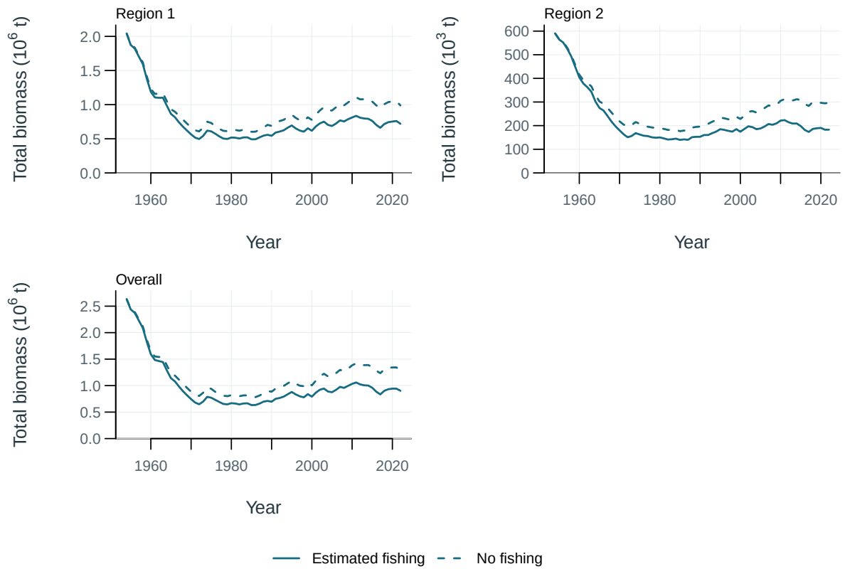
Figure 53: Total biomass under estimated fishing (solid) and the dynamic no-fishing counterfactual (dashed), by region and overall.
