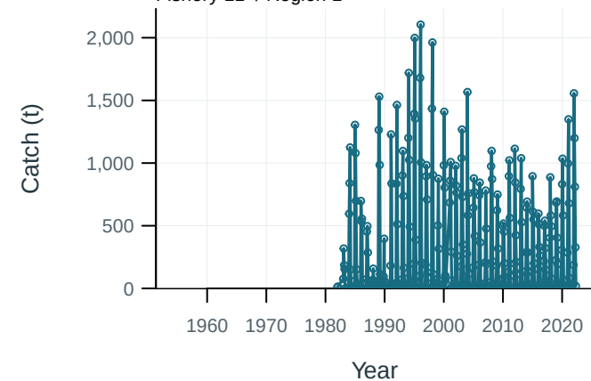
Fishery 11 / Region 1
