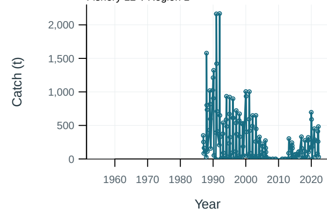
Fishery 12 / Region 1
