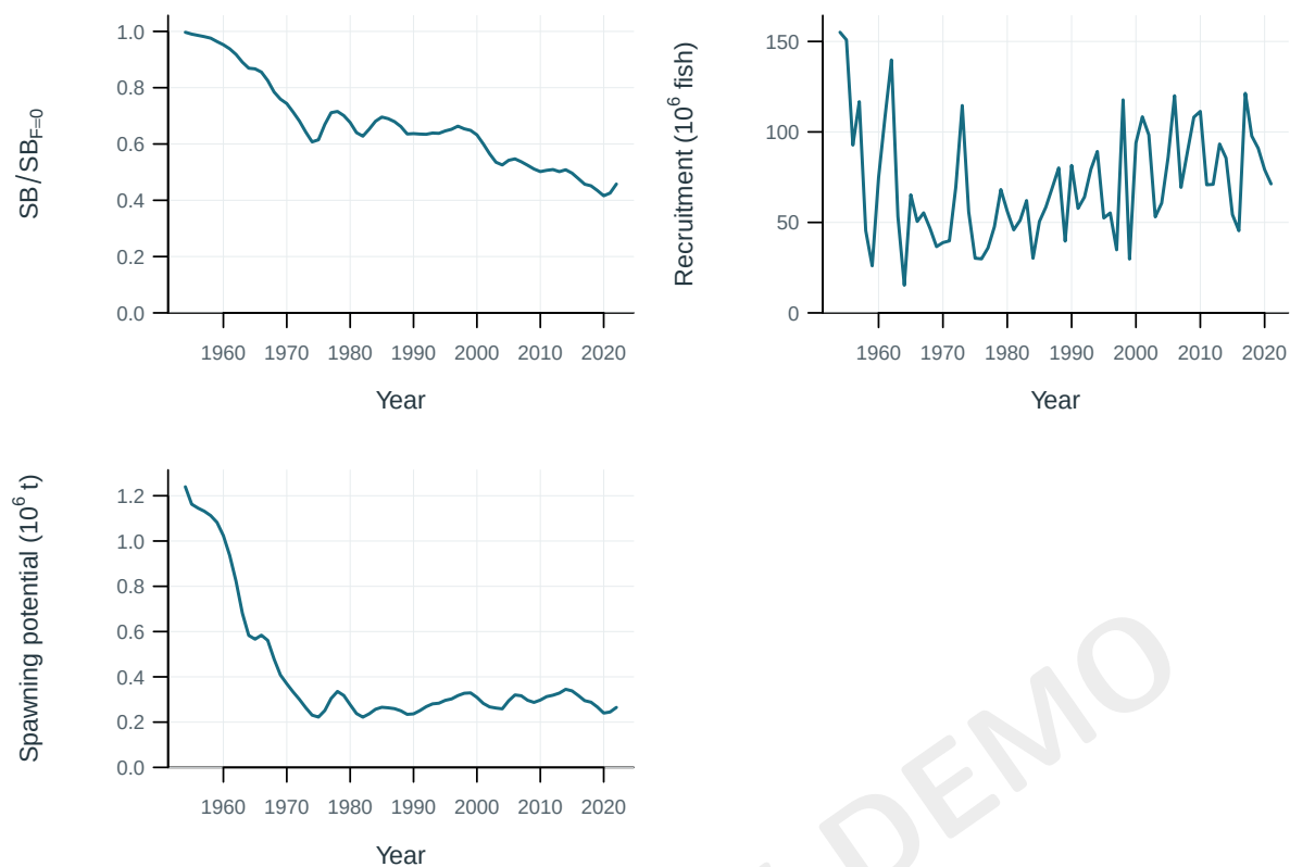
Figure 28: Estimated population trajectories.
