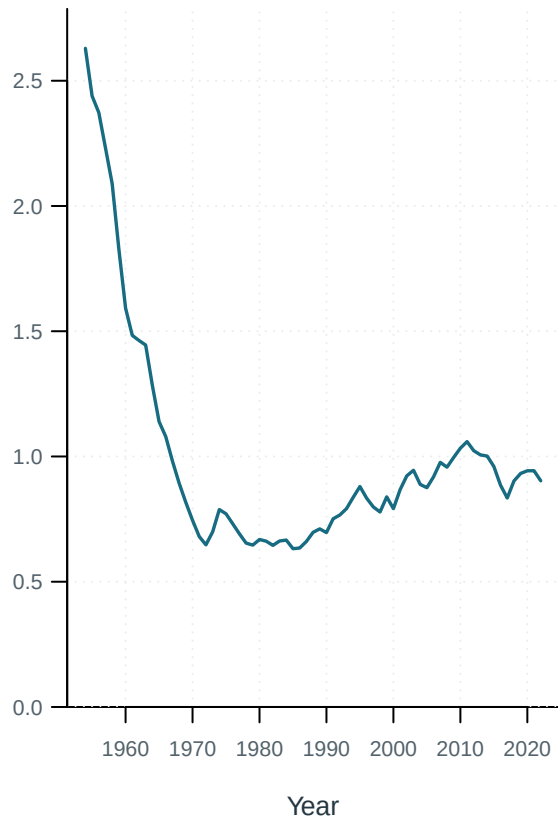
Dynamic unfished total biomass ( 10^6 t)
