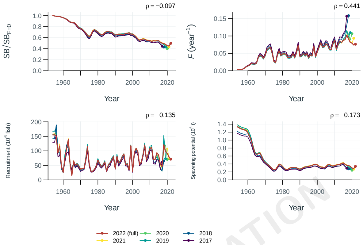
Figure 12: Population trajectories for the full-data fit and retrospective peels. Points mark terminal years; \rho is Mohn's mean terminal relative difference for peels passing the recorded numerical checks.
