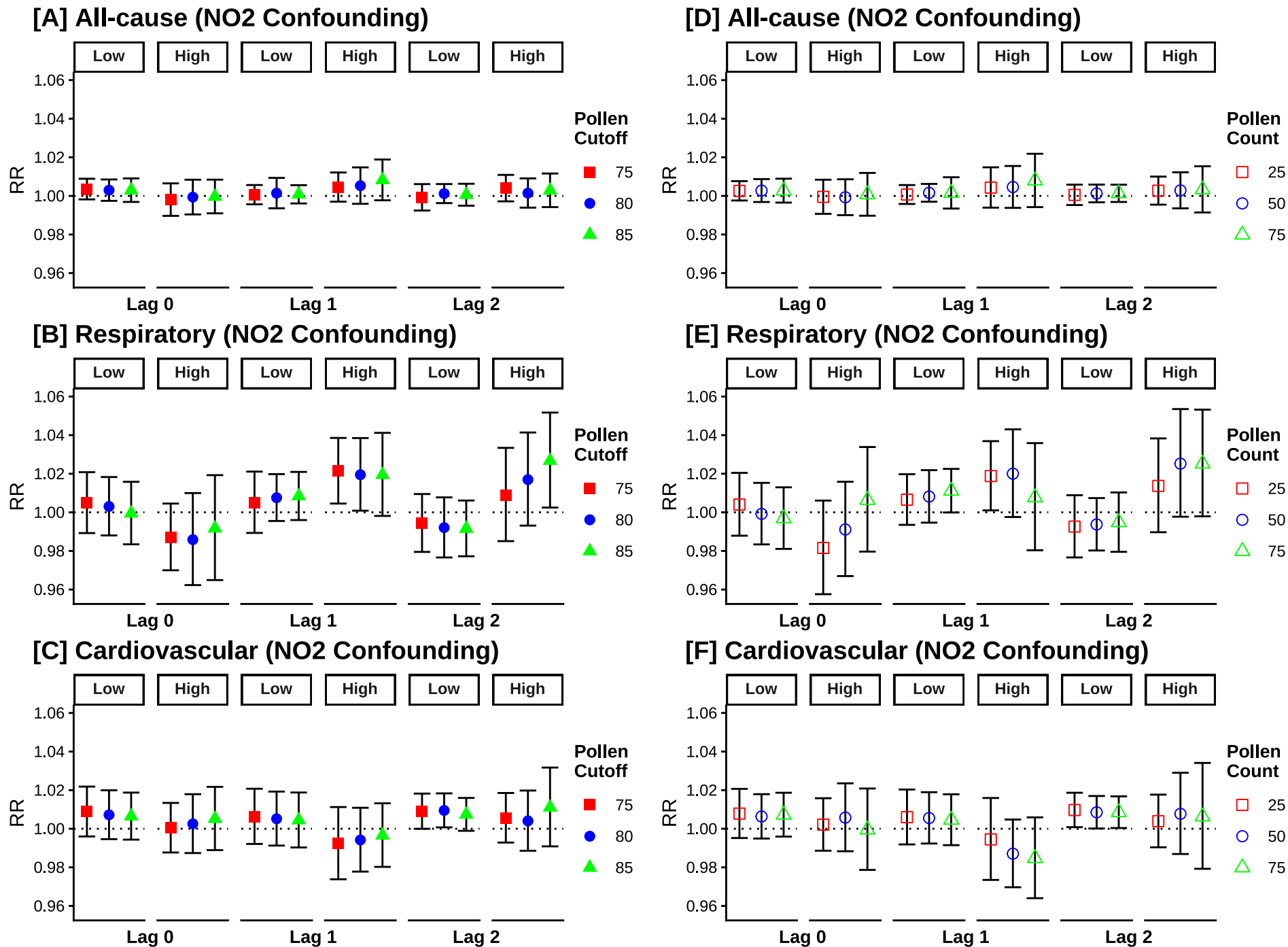
Figure S4. Two-pollutant model with NO 2 as the confounder. Association between SPM and all-cause respiratory and cardiovascular mortality by quantiles (low or high) determined by levels of pollen cutoffs (75 th , 80 th , 85 th ) and count (25, 50, 75 grains per cm 2 ) during the spring months (February to April) from 1989 to 2014. RR on the y-axis is defined as the relative risk per interquartile range mean (IQR) increase. Results are pooled from random-effects meta-analysis.
