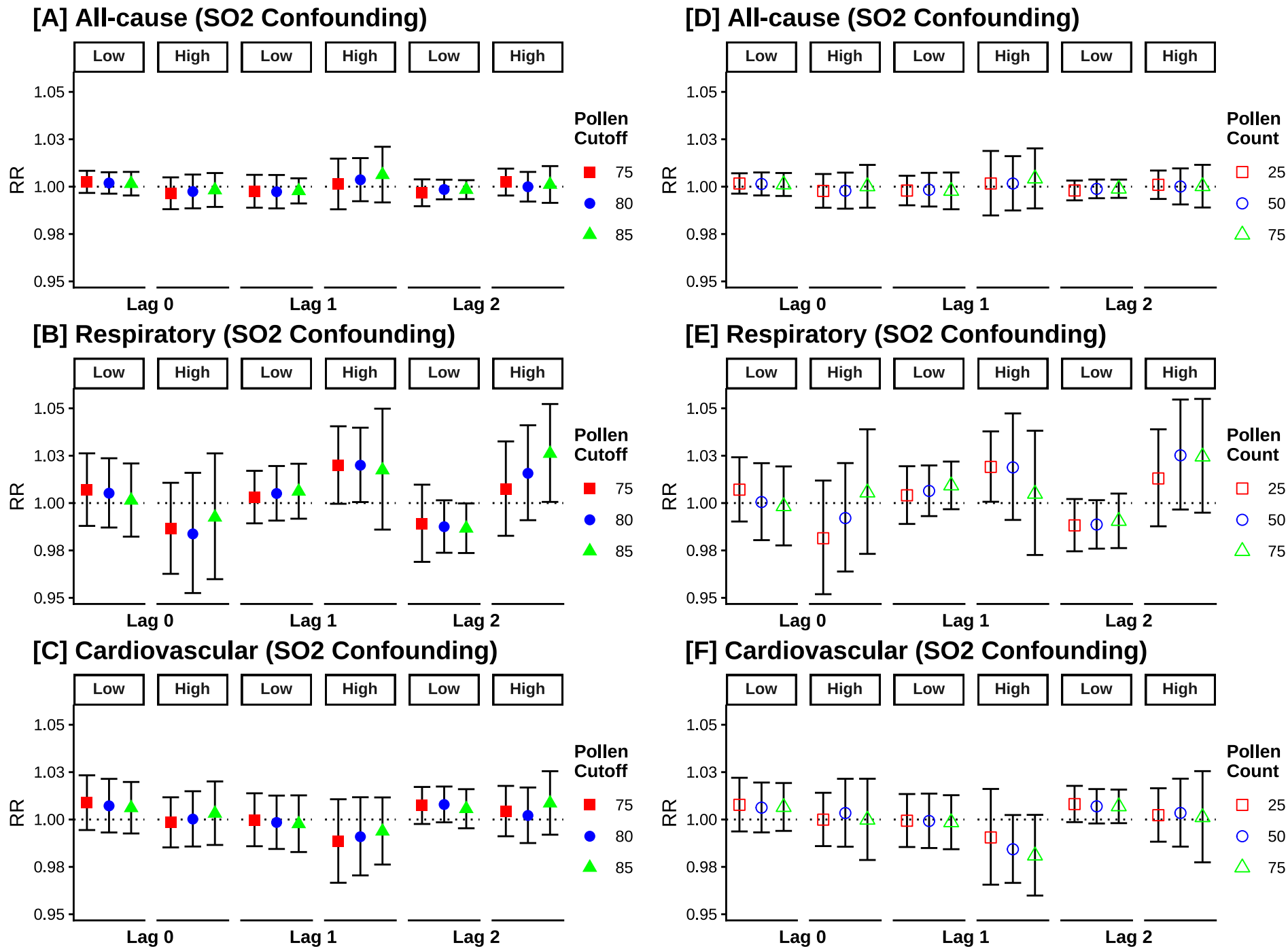
Figure S5. Two-pollutant model with SO 2 as the confounder. Association between SPM and all-cause, respiratory and cardiovascular mortality by quantiles (low or high) determined by levels of pollen cutoffs (75 th , 80 th , 85 th ) and count (25, 50, 75 grains per cm 2 ) during the spring months (February to April) from 1989 to 2014. RR on the y-axis is defined as the relative risk per interquartile range mean (IQR) increase. Results are pooled from random-effects meta-analysis.
