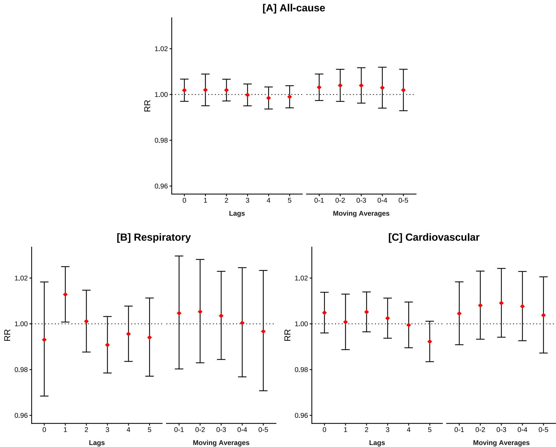
Figure 2. Association between SPM and all-cause, respiratory and cardiovascular mortality during the spring months (February to April) from 1989 to 2014. RR on the y-axis is defined as the relative risk per interquartile range mean (IQR) increase. Results are pooled from random-effects meta-analysis.
