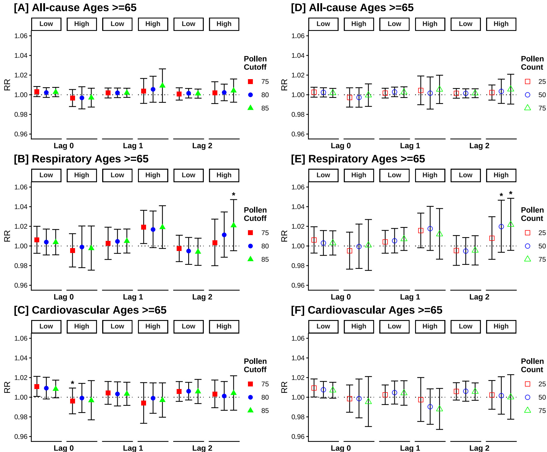
Figure S3. Association between SPM and all-cause, respiratory and cardiovascular mortality of ages 65 and above by quantiles (low or high) determined by levels of pollen cutoffs (75 th , 80 th , 85 th ) and count (25, 50, 75 grains per cm 2 ) during the spring months (February to April) from 1989 to 2014. RR on the y-axis is defined as the relative risk per interquartile range mean (IQR) increase. Results are pooled from random-effects meta-analysis.
