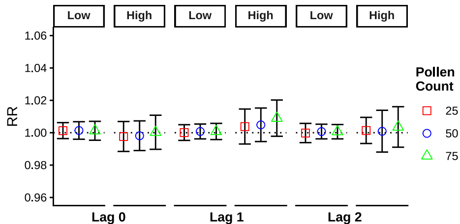
[E] Respiratory (NO2 Confounding)
