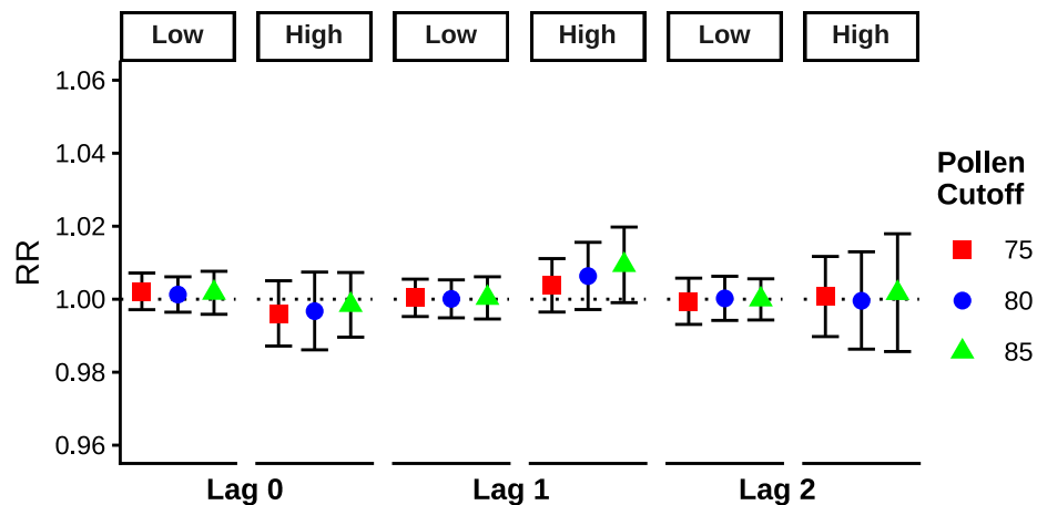
[B] Respiratory (NO2 Confounding)
