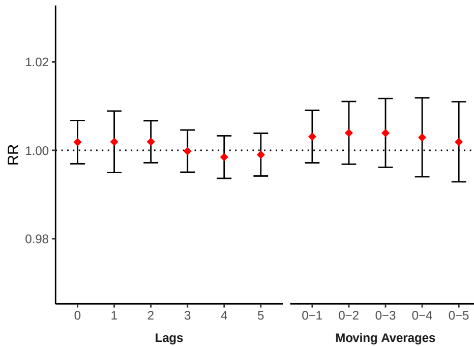
[A] All-cause
