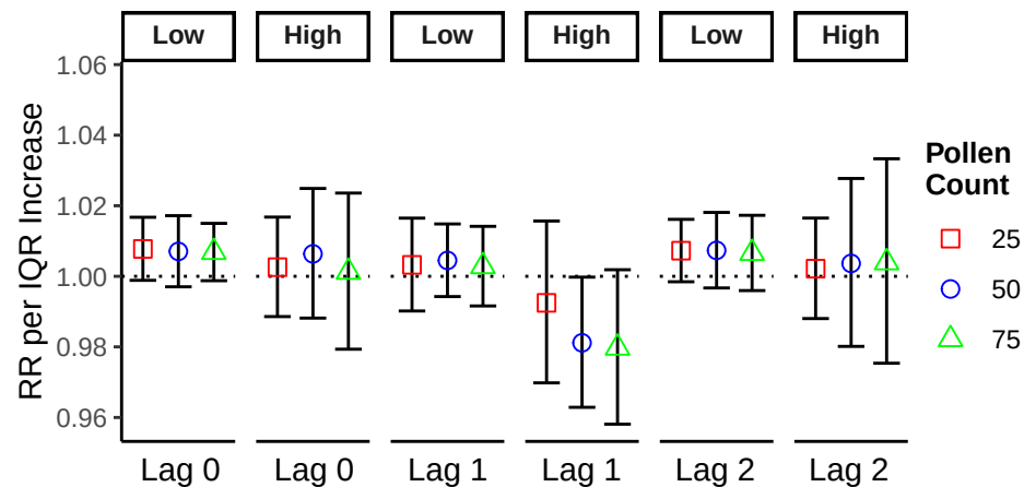
[F] Cardiovascular Ages \geq 65
