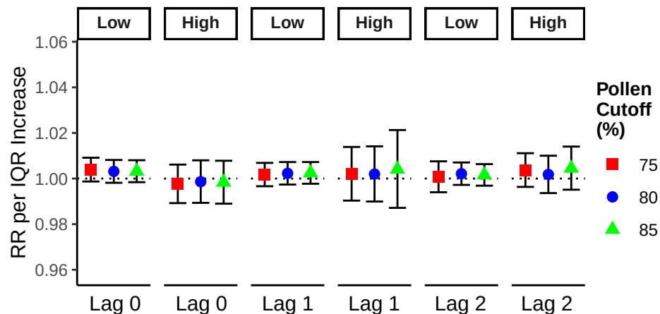
[B] Respiratory Ages \geq 65
