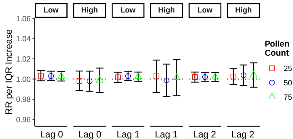
[E] Respiratory Ages \geq 65
