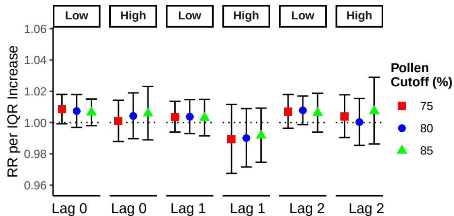
[C] Cardiovascular Ages \geq 65
