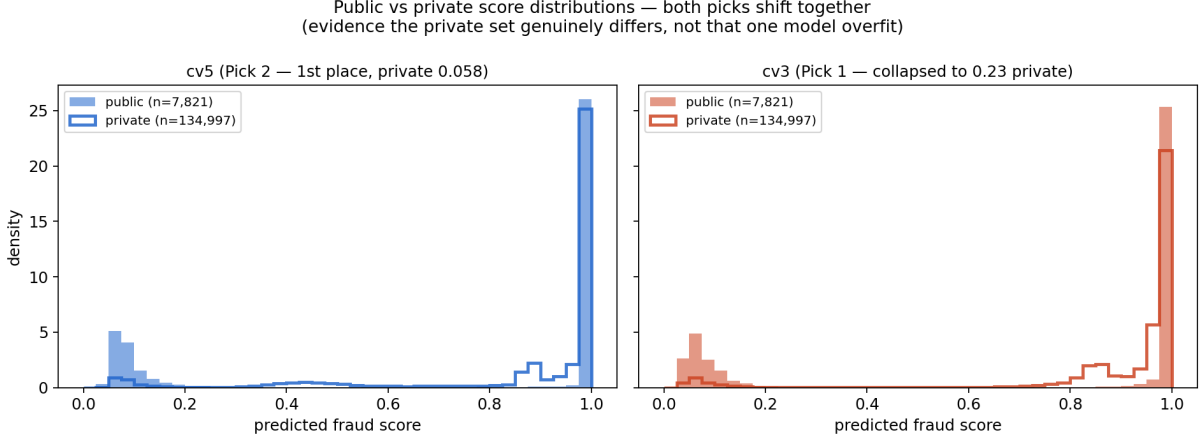
Figure 6: Public vs. private prediction distributions for both picks. Both shift together, consistent with a genuinely different private-set composition rather than model-specific overfitting; see Section 5.1.
