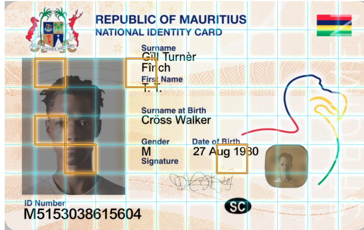
Figure 3: The per-patch MIL head scores many small patches of the document independently (cyan grid) and drives the image-level decision from the most suspicious local regions (amber). Local forgery cues — blend seams, splice boundaries, compression discontinuities — transfer across document types, whereas global layout does not; this is what pushes the model toward type-agnostic evidence.
