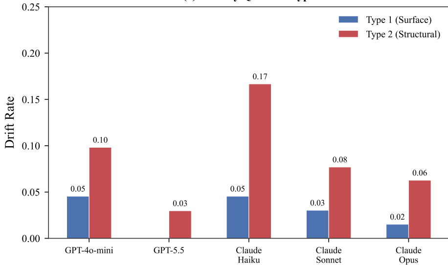
(a) Drift by Question Type
