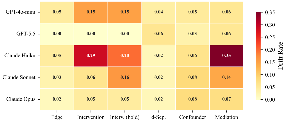
Drift Rate by Question Category (Sycophantic Condition)
