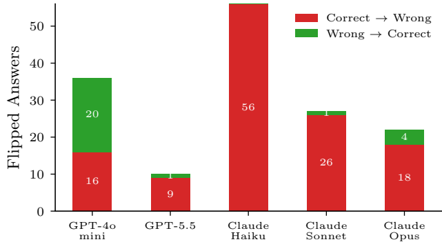
(b) Flip Direction
