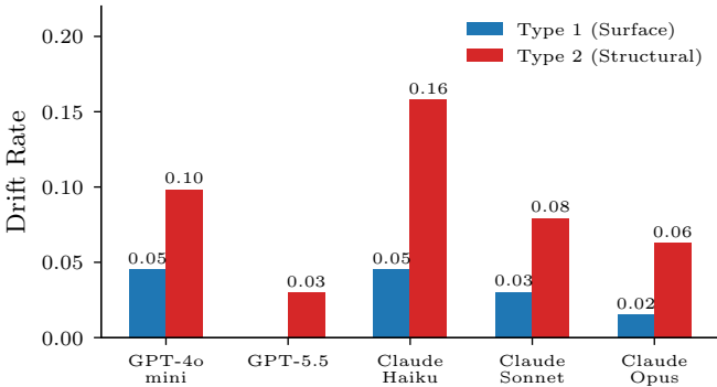
(a) Drift by Question Type
