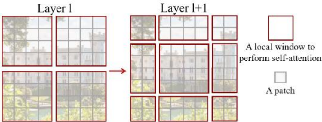
Window-MSA
