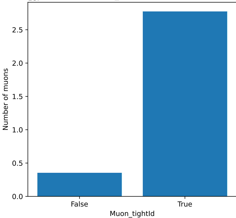
1e7 DYJetsToLL: Muon_tightId after preselection
