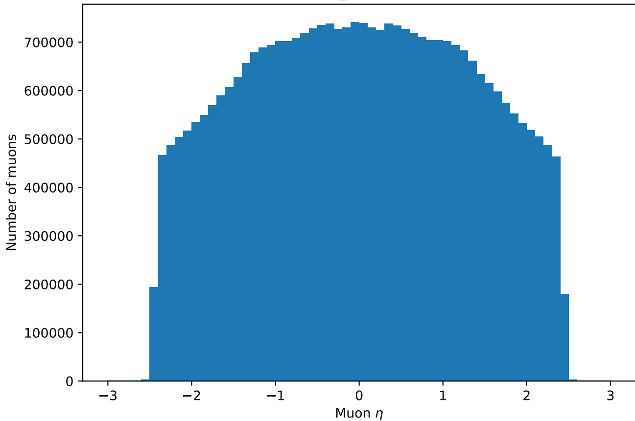
DYJetsToLL: Muon_eta after preselection
