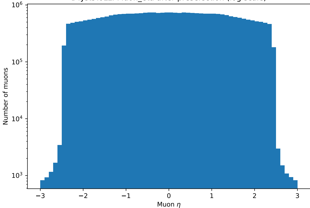
DYJetsToLL: Muon_eta after preselection (log scale)
