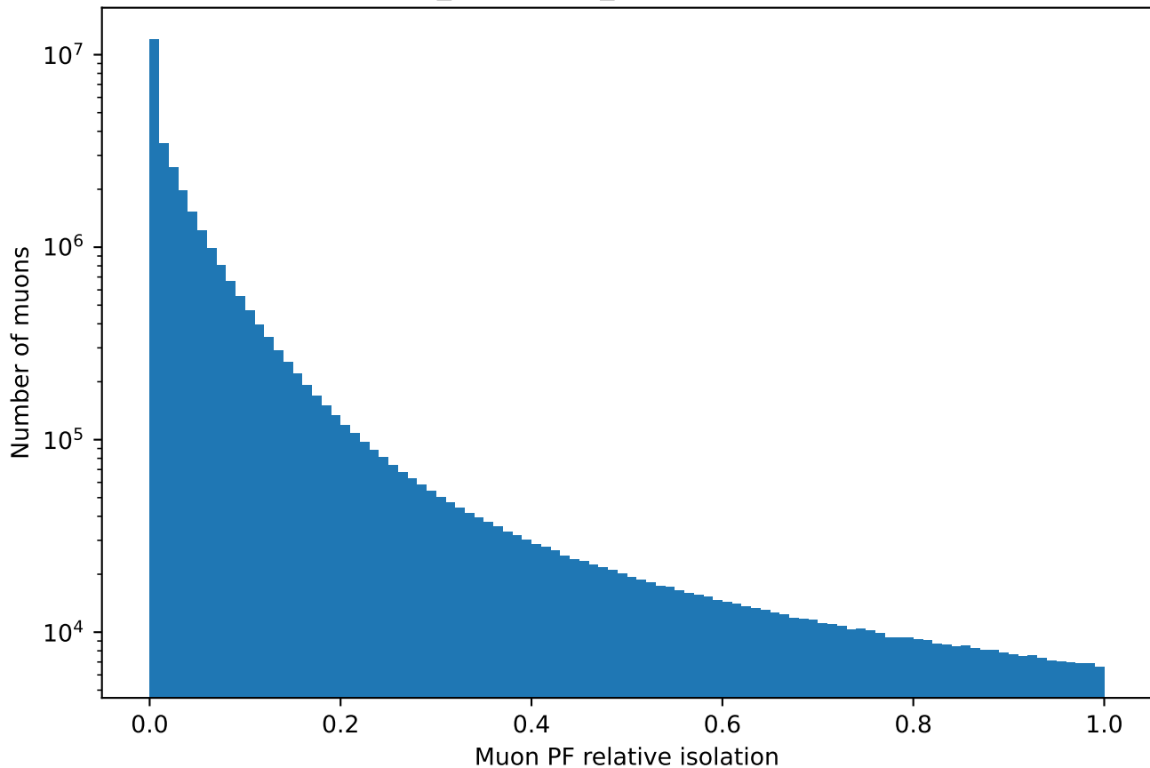
DYJetsToLL: Muon_pfRelIso04_all after preselection (log scale)
