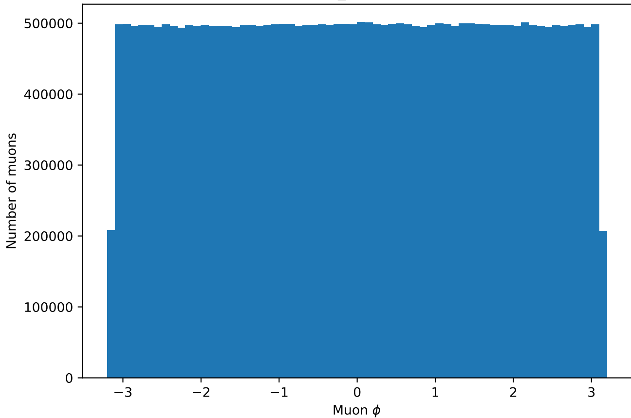
DYJetsToLL: Muon_phi after preselection
