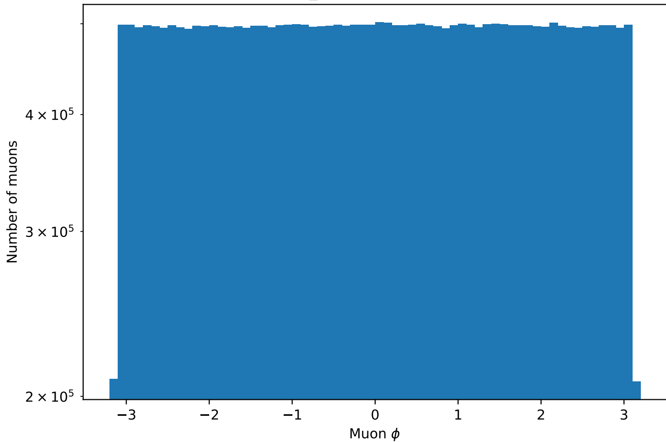
DYJetsToLL: Muon_phi after preselection (log scale)
