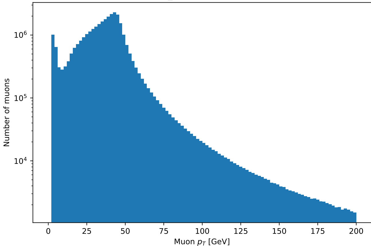
DYJetsToLL: Muon_pt after preselection (log scale)
