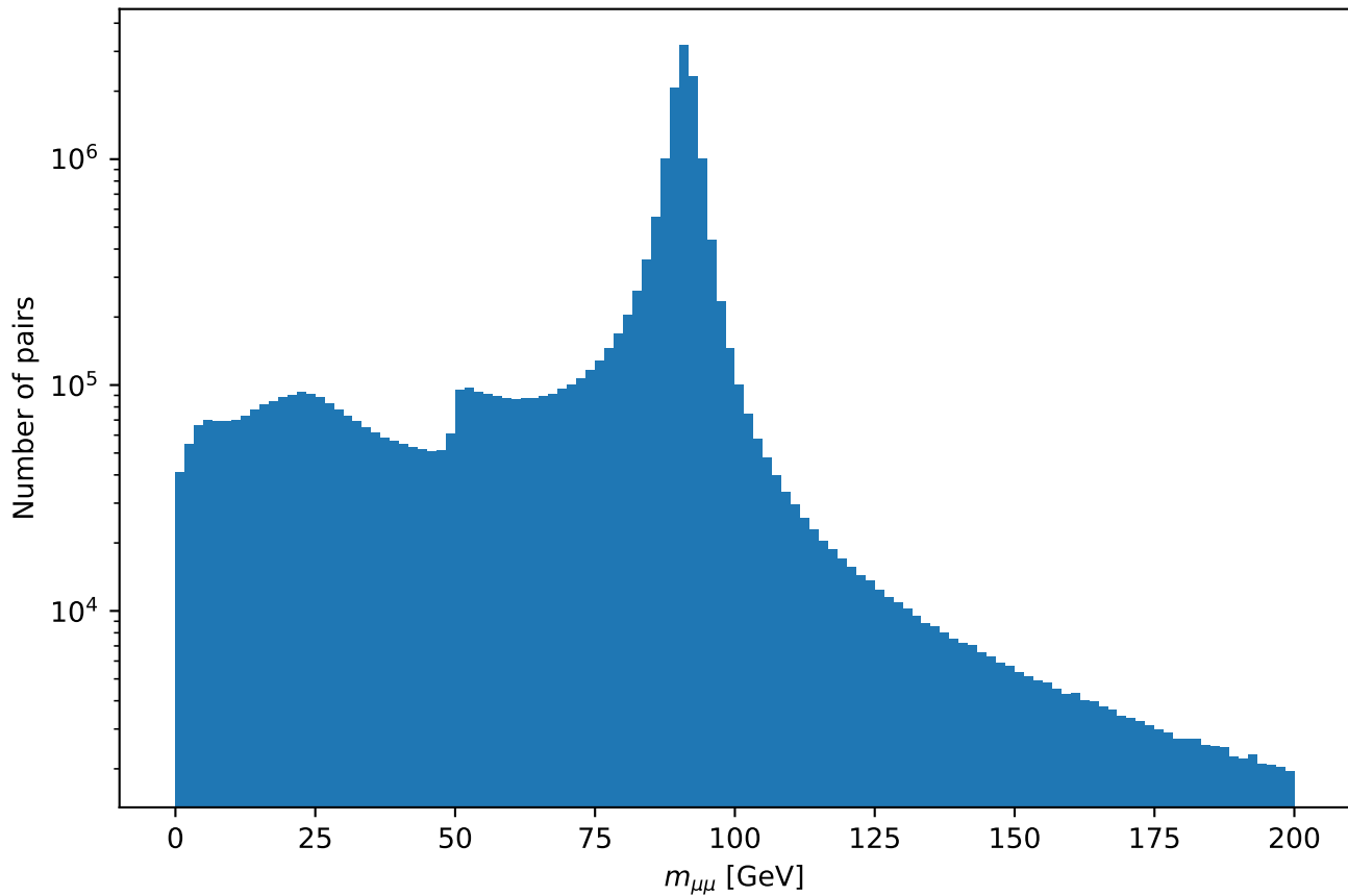
DYJetsToLL: opposite-charge dimuon mass (log scale)
