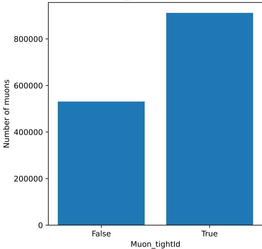
TTbar: Muon_tightId after preselection
