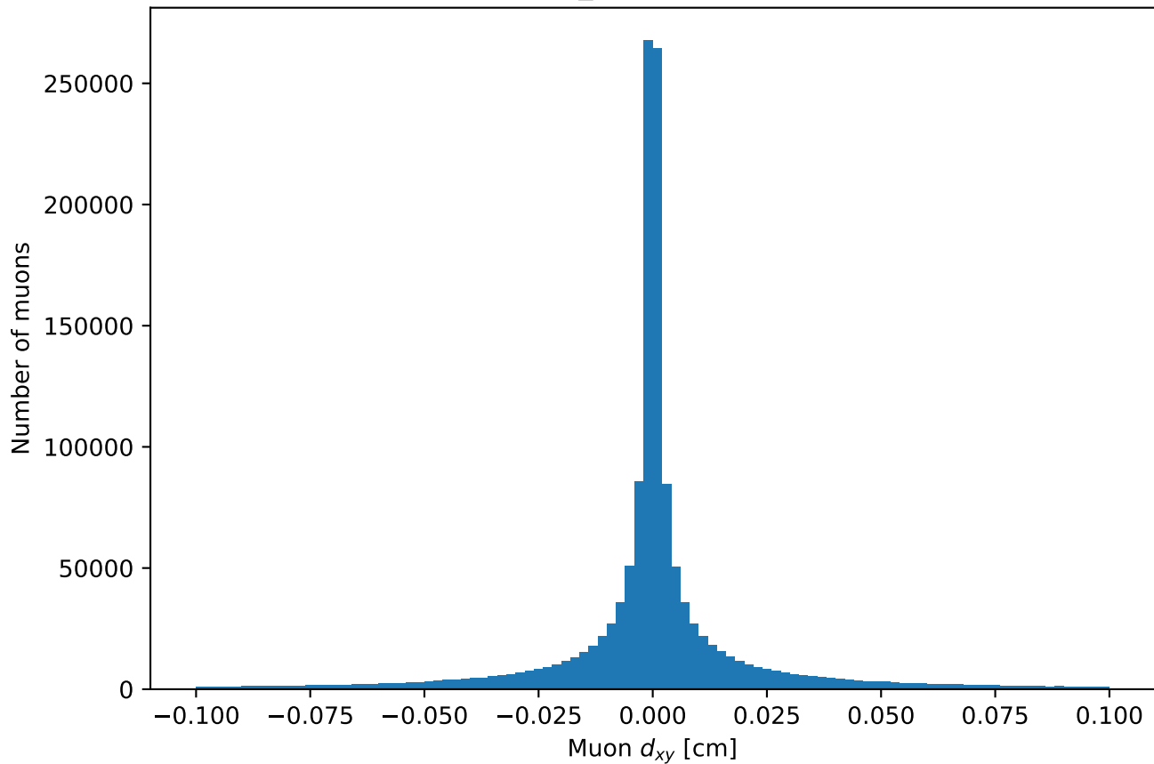
T\bar{T} bar: Muon d_{xy} after preselection
