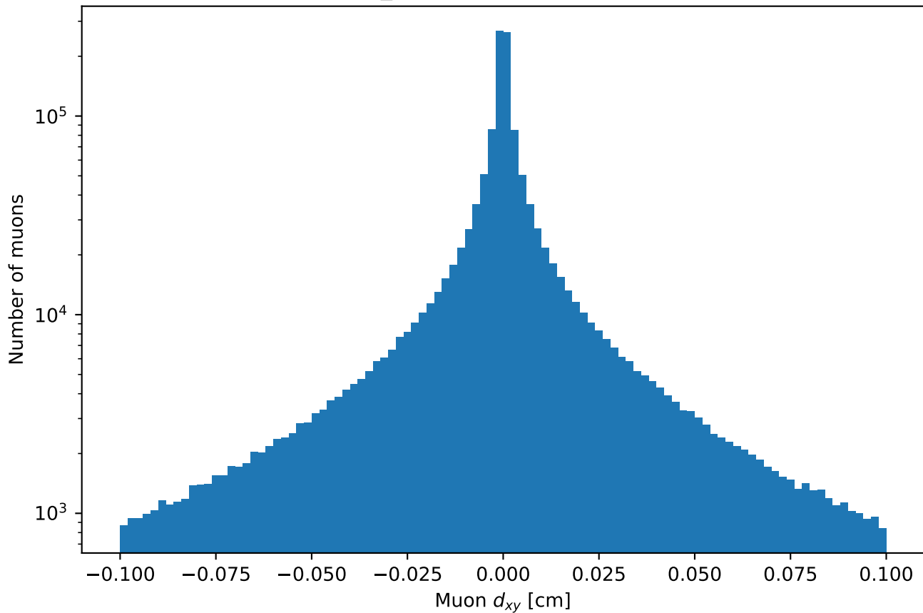
TTbar: Muon_dxy after preselection (log scale)
