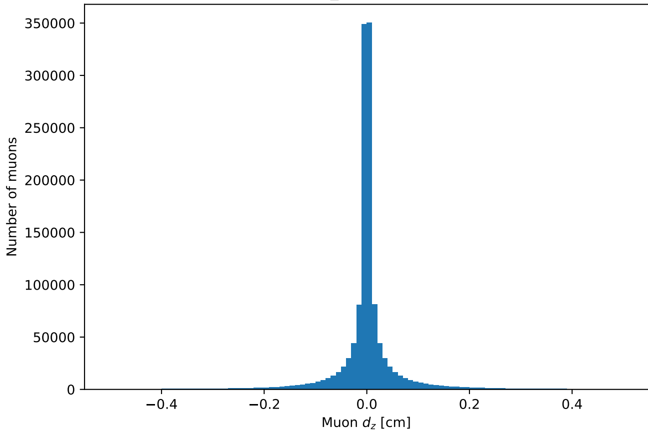
TTbar: Muon_dz after preselection
