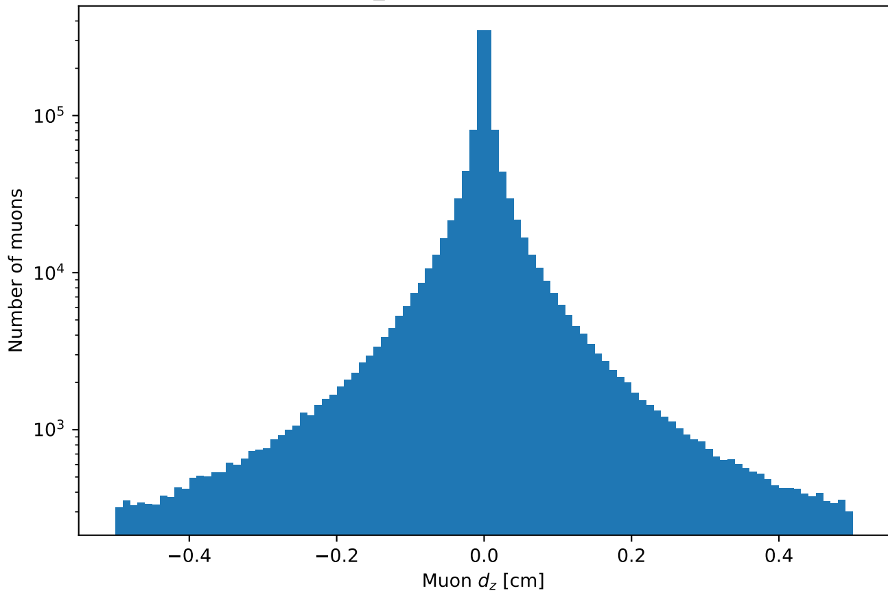
T\bar{T} bar: Muon d_z after preselection (log scale)
