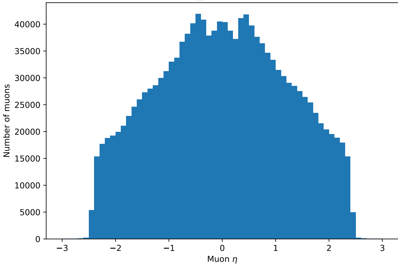
T\bar{T} bar: Muon_eta after preselection
