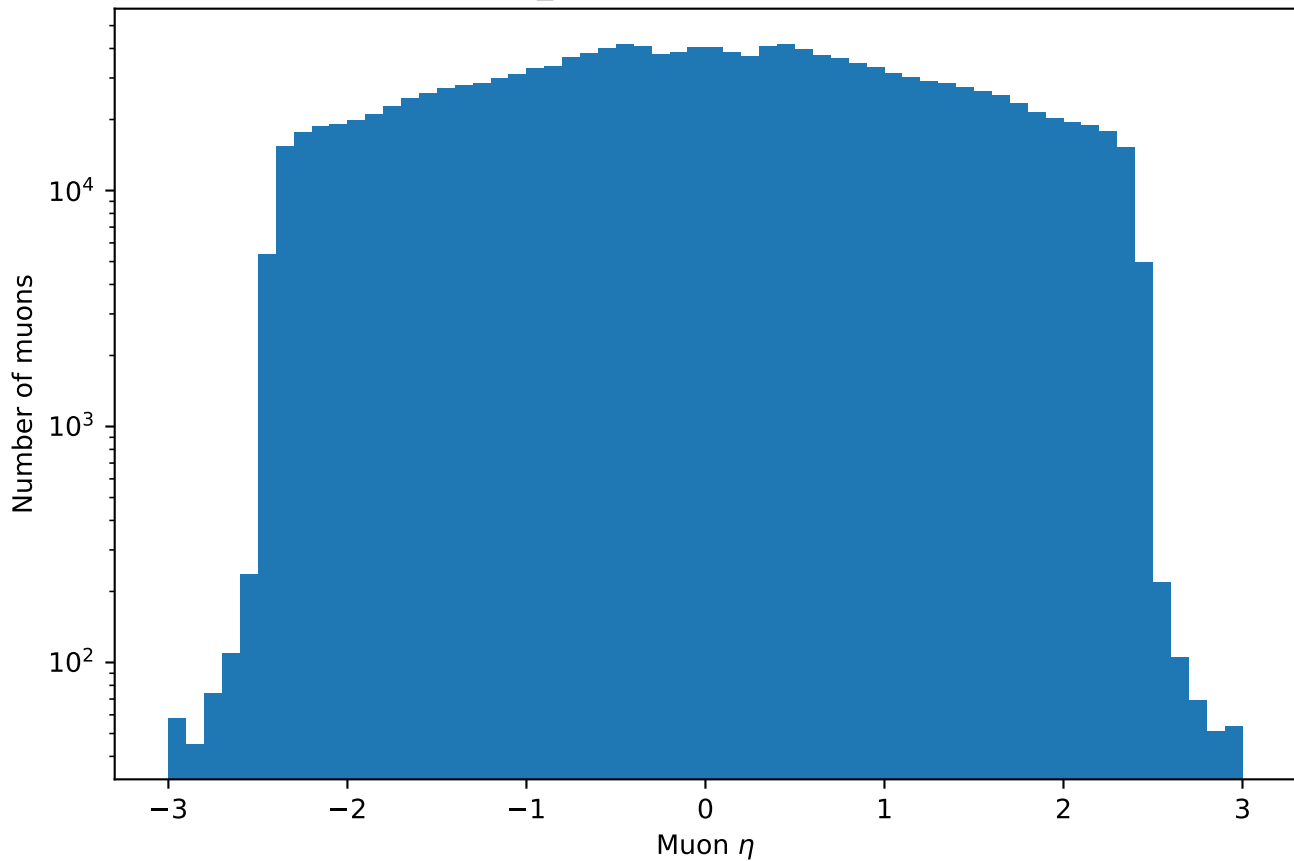
TTbar: Muon_eta after preselection (log scale)
