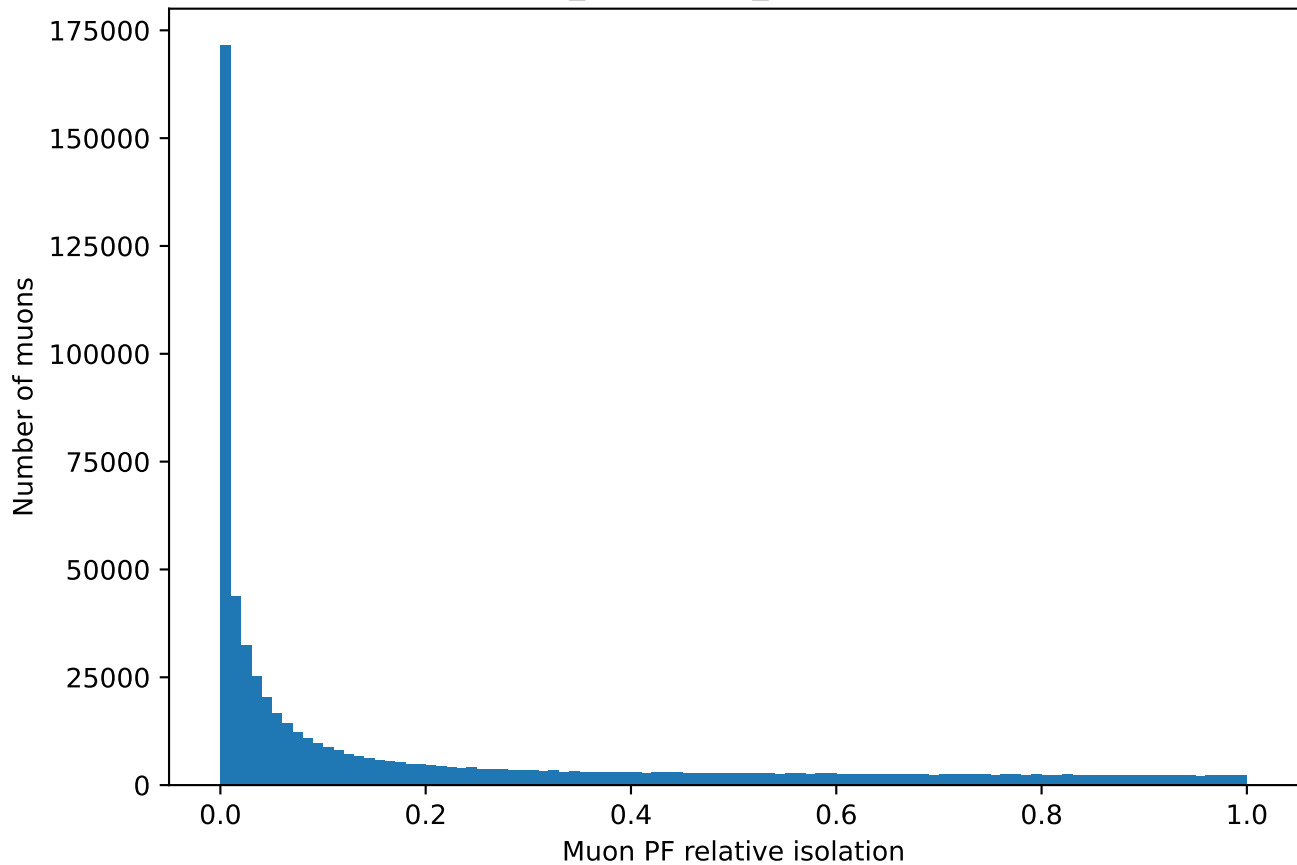
T\bar{T} bar: Muon_pfRelIso04_all after preselection
