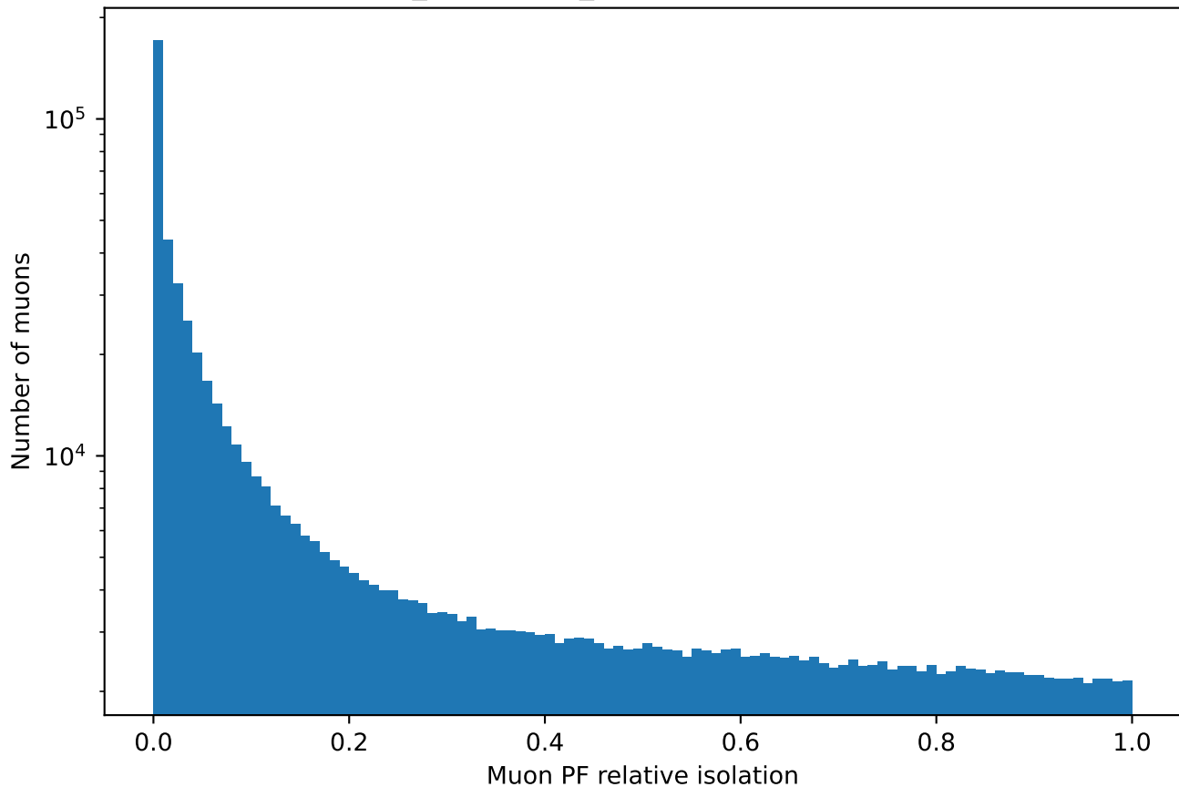
T\bar{T} bar: Muon_pfRelIso04_all after preselection (log scale)
