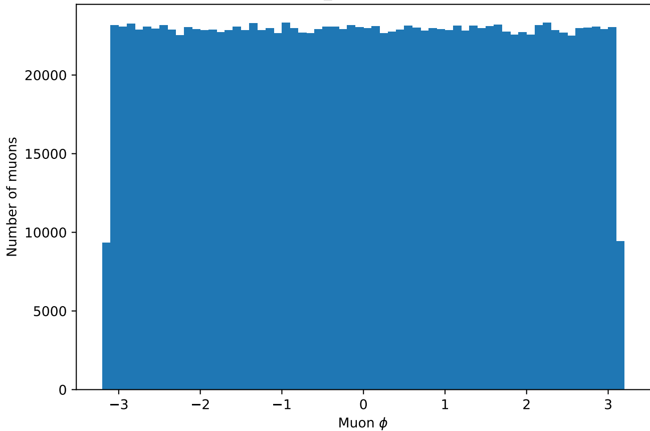
TTbar: Muon_phi after preselection
