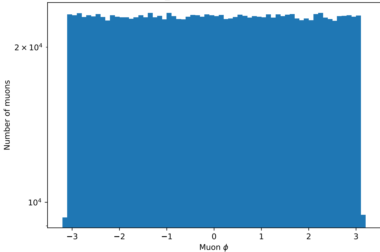
TTbar: Muon_phi after preselection (log scale)
