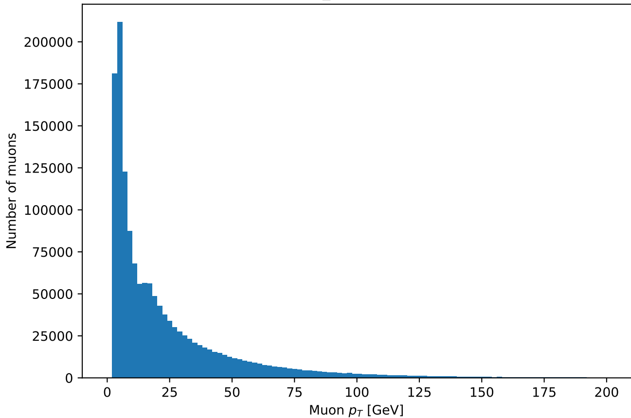
T\bar{T} bar: Muon p_T after preselection
