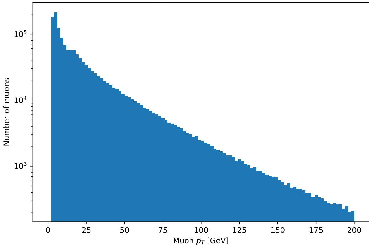
TTbar: Muon_pt after preselection (log scale)
