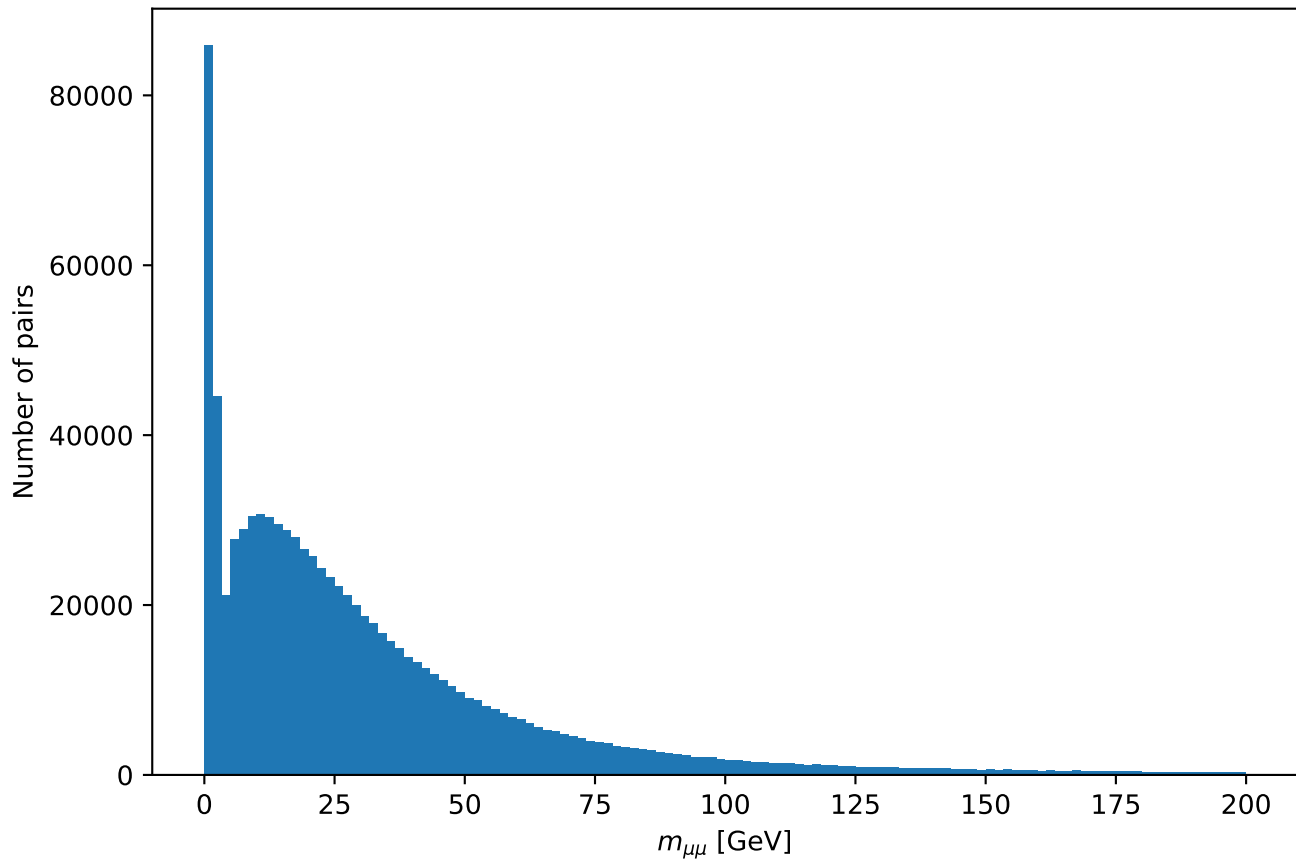
T\bar{T} : opposite-charge dimuon mass
