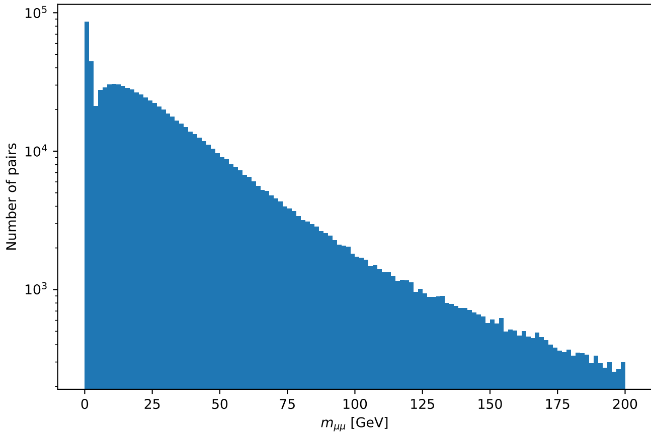
T\bar{T} : opposite-charge dimuon mass (log scale)
