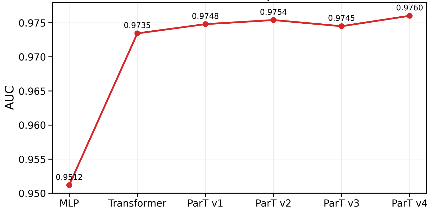
Model AUC comparison
