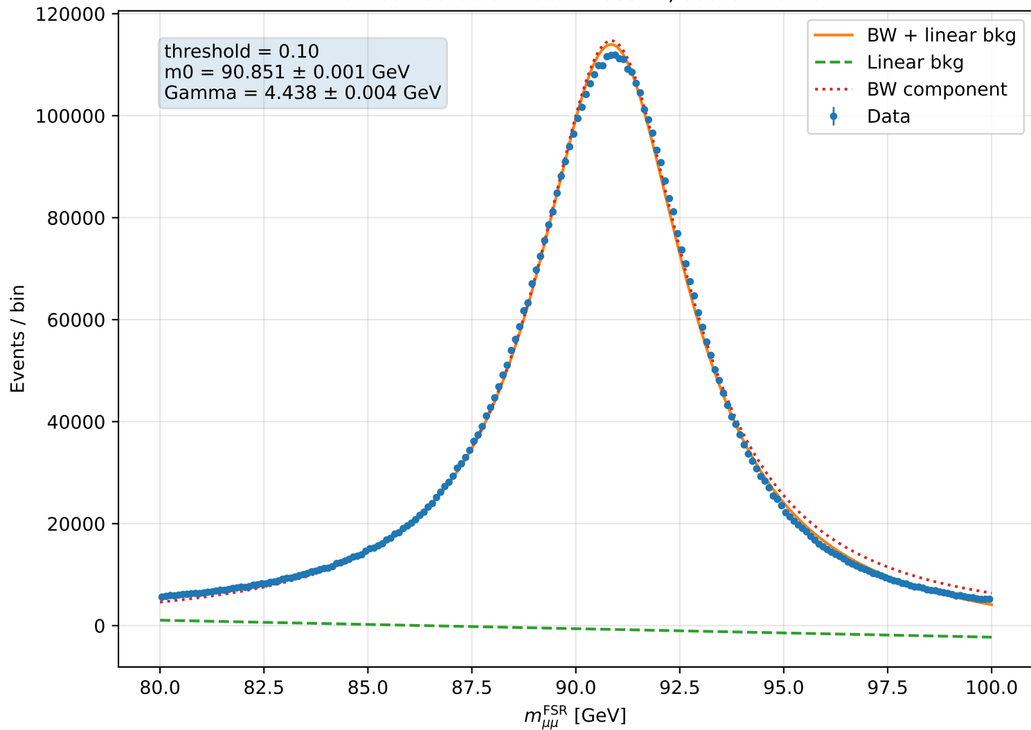
FSR corrected dimuon mass fit, score &gt; 0.10
