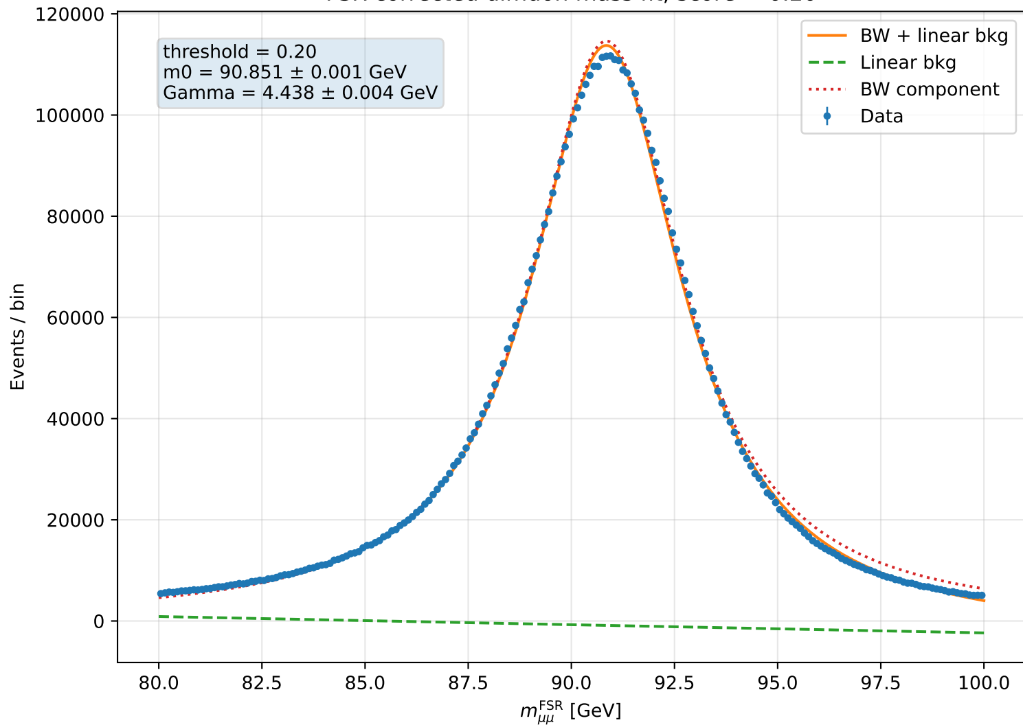
FSR corrected dimuon mass fit, score &gt; 0.20
