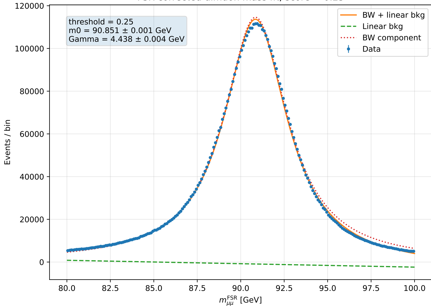
FSR corrected dimuon mass fit, score &gt; 0.25
