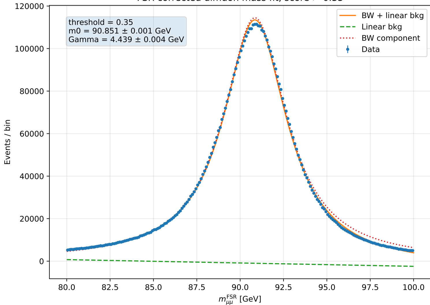
FSR corrected dimuon mass fit, score &gt; 0.35
