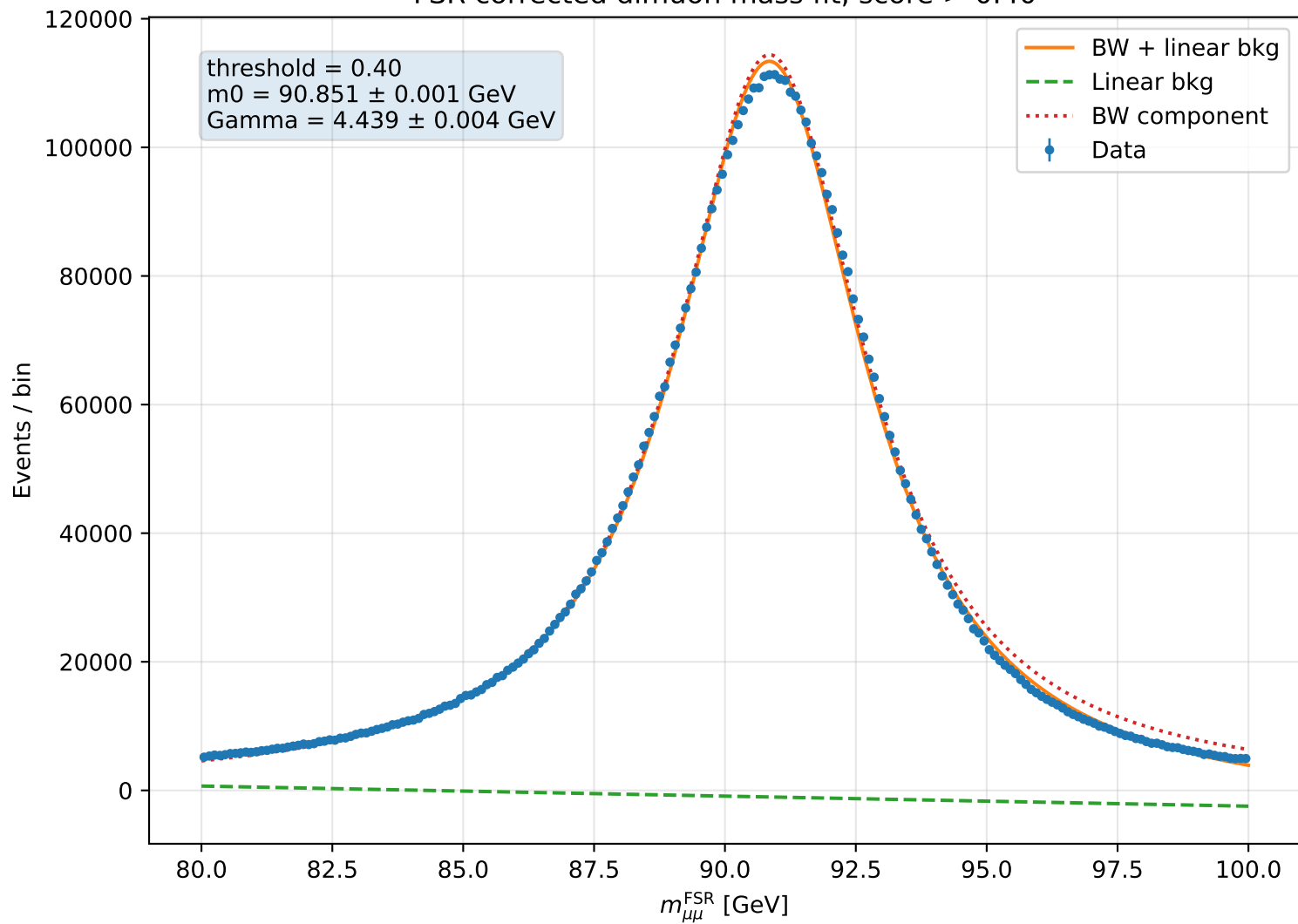
FSR corrected dimuon mass fit, score &gt; 0.40
