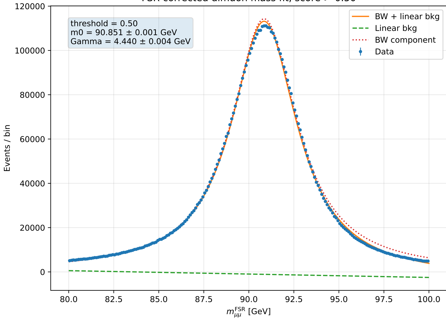
FSR corrected dimuon mass fit, score &gt; 0.50
