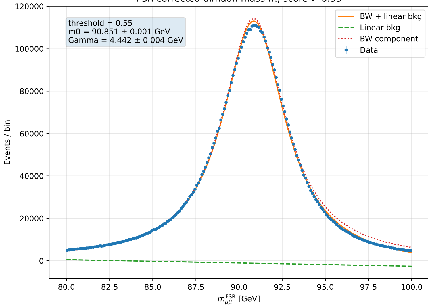
FSR corrected dimuon mass fit, score &gt; 0.55
