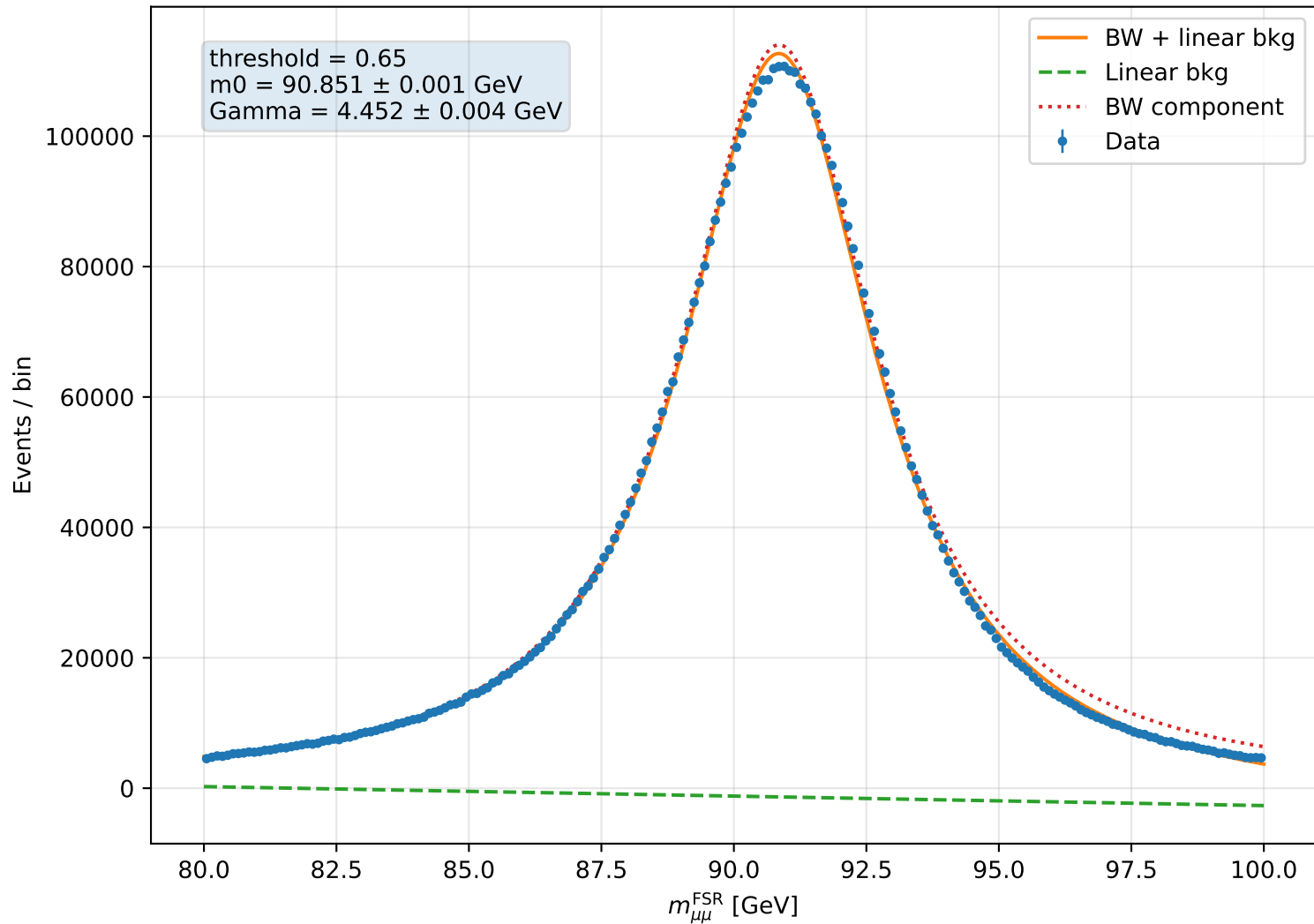
FSR corrected dimuon mass fit, score &gt; 0.65
