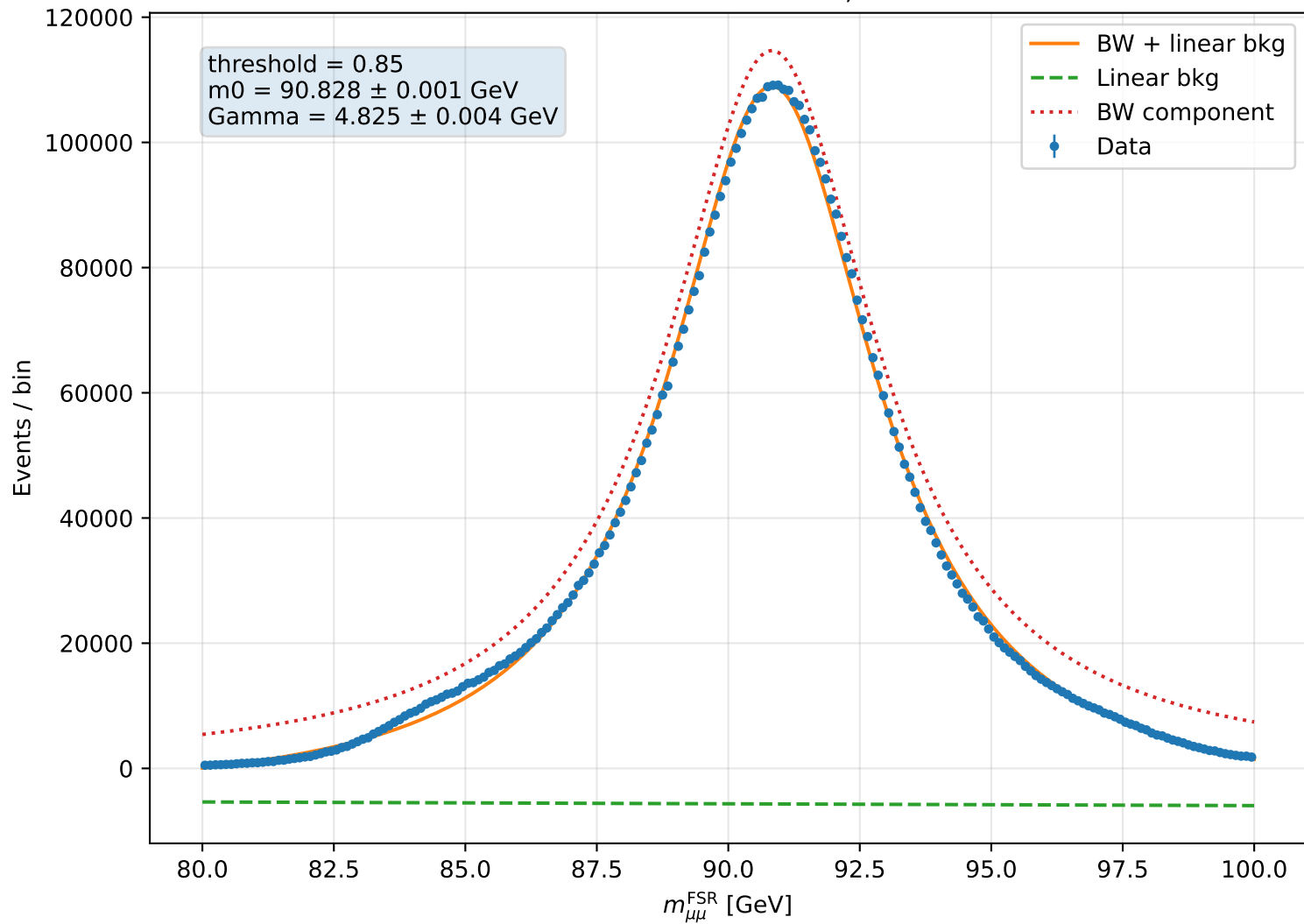
FSR corrected dimuon mass fit, score &gt; 0.85
